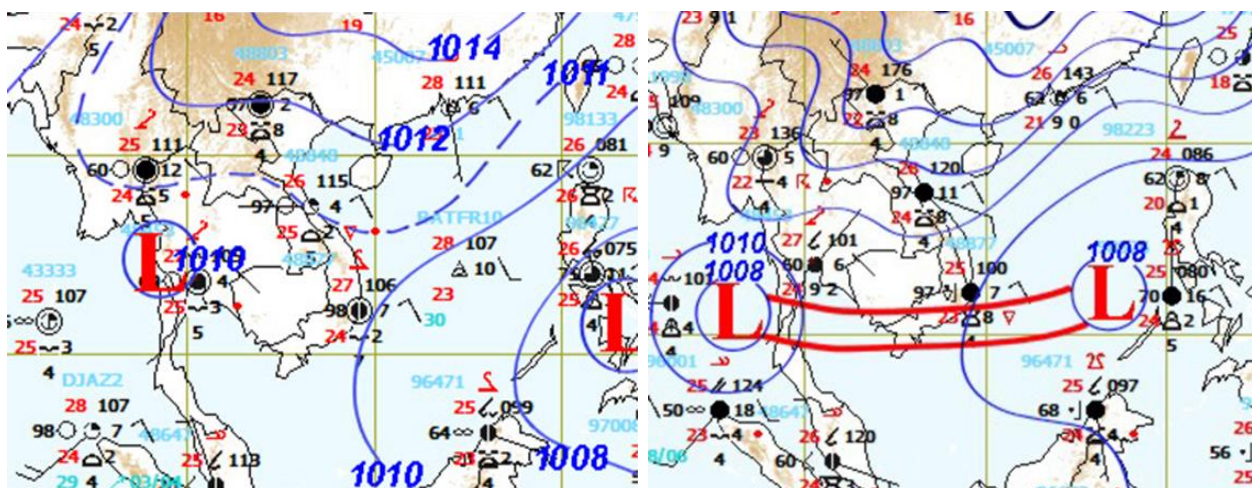
Figure 1: Weather map for 29 th September 2014
